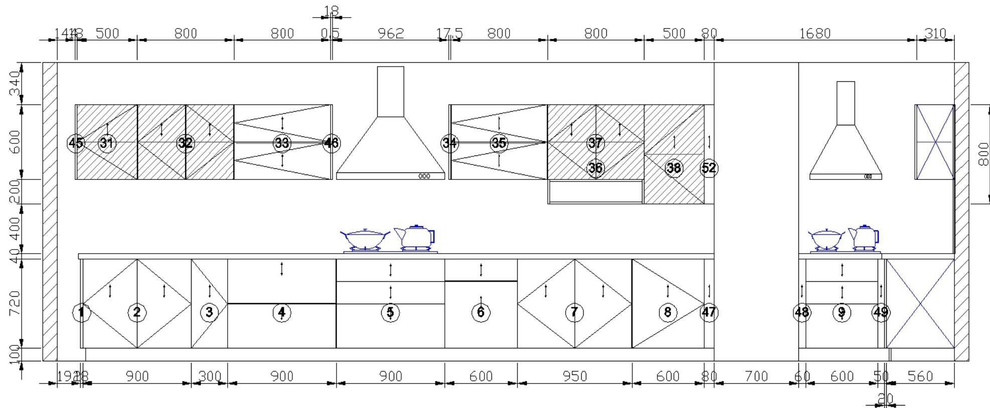
A View elevation drawing
