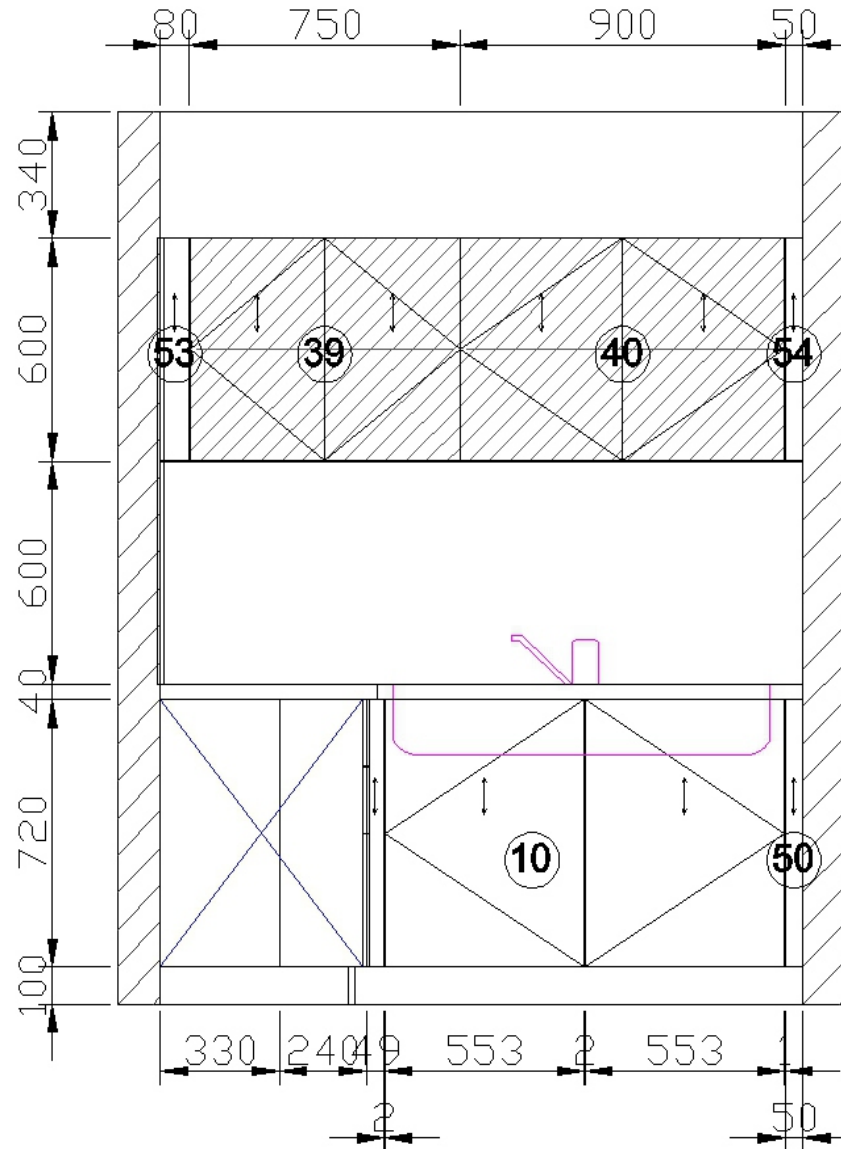
B View elevation drawing
